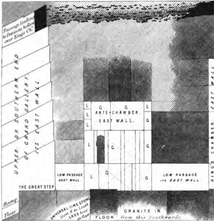
VERTICAL MERIDIAN SECTION from G Gallery through ANTE-CHAMBER to Kings Ch Looking Eastward
